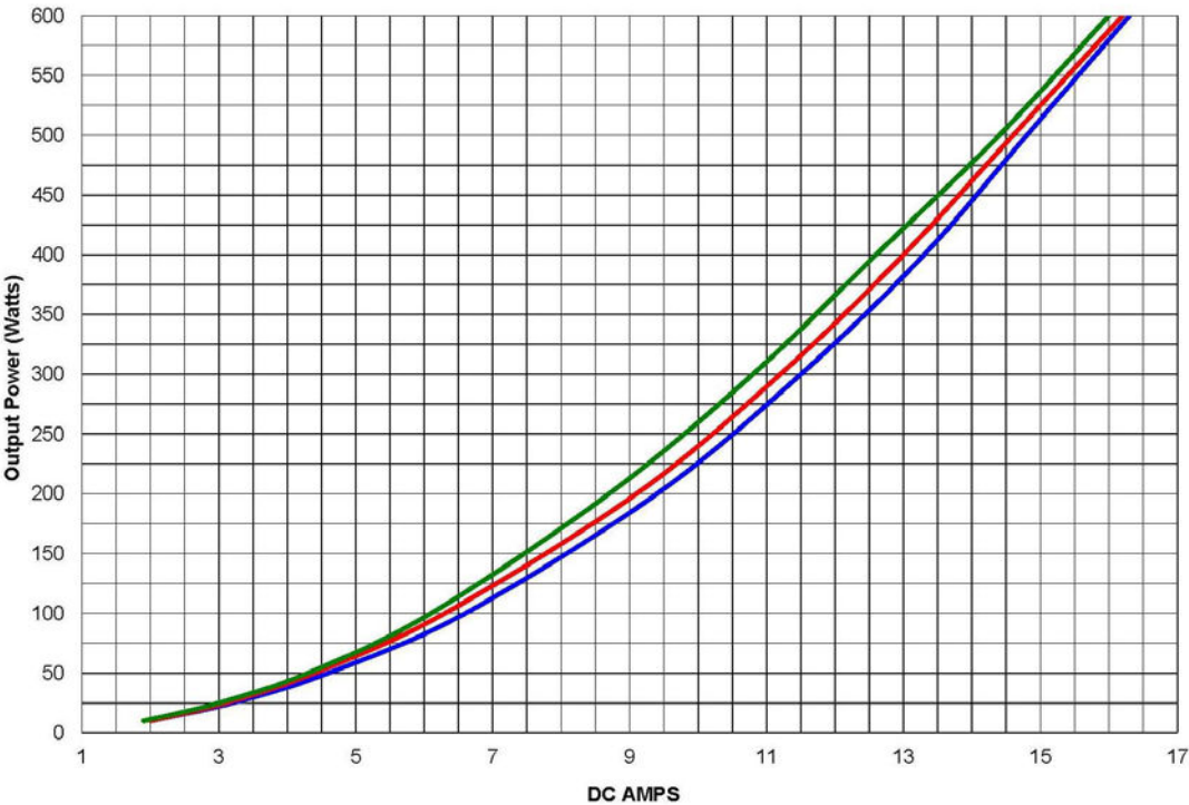
DC Amps Vs Output Power @ 48VDC; BLF184XR 150ma bias
