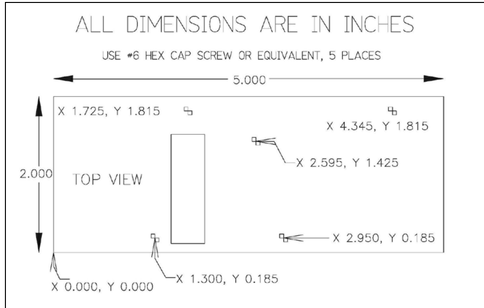
Amplifier Mechanical Drawing: Figure 1
